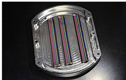
Beam splitter used in aerial cameras
